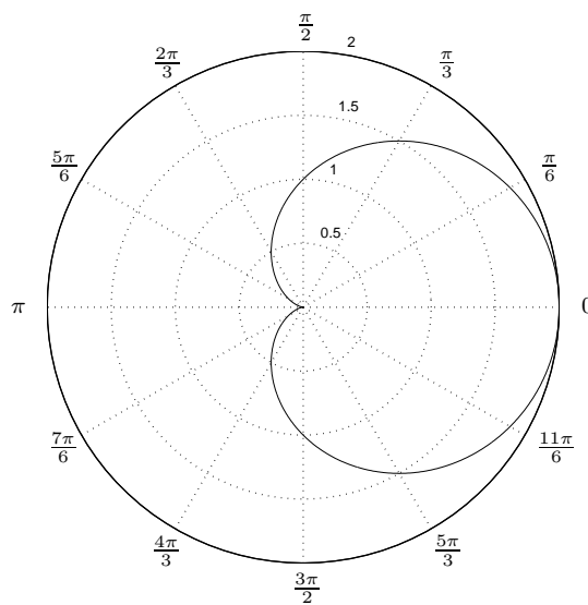
r = 1 + \cos \theta (Cardioid)
