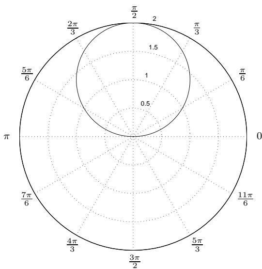
r = 2 \sin \theta (Circle)
